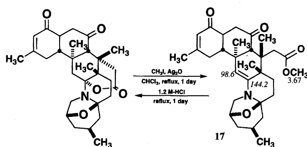
Fig. 17. Esterification of norzoanthamine.
